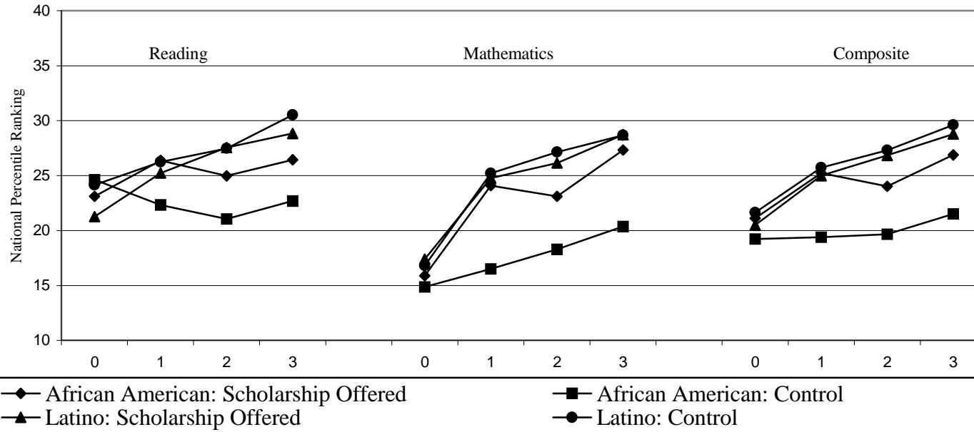
FIGURE E-1 ADJUSTED TEST SCORE MEANS FOR AFRICAN AMERICANS AND LATINOS
