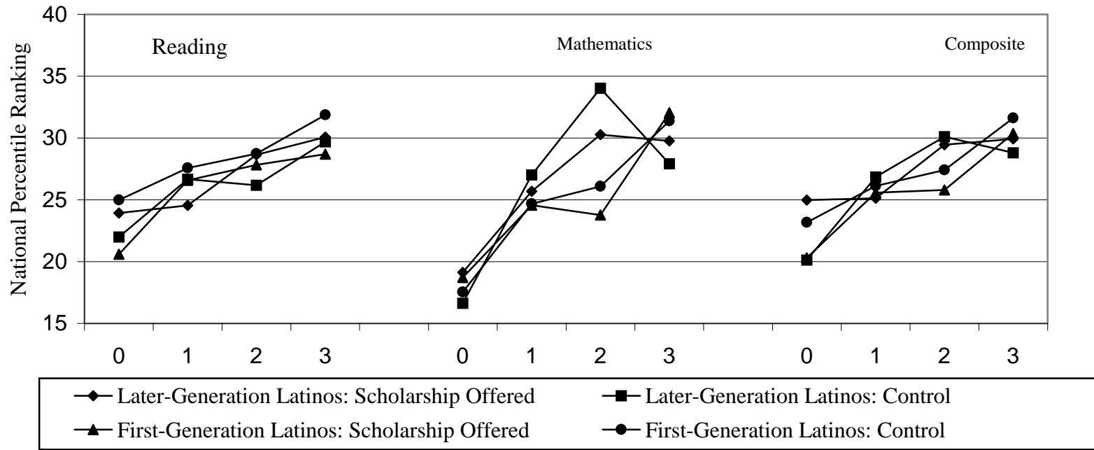
FIGURE E-2 ADJUSTED TEST SCORE MEANS FOR FIRST AND LATER GENERATION LATINOS
